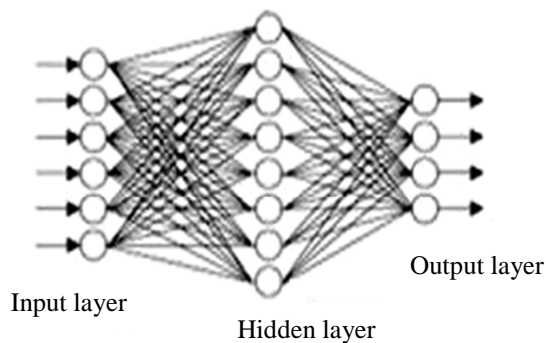
Fig. 2. Schematic diagram of ANN model with 6-8-4 structure
