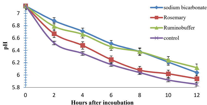
Fig. 2. Comparison of the effect of Rumenobuffer, sodium bicarbonate, Rosemary powder on instantaneous pH
